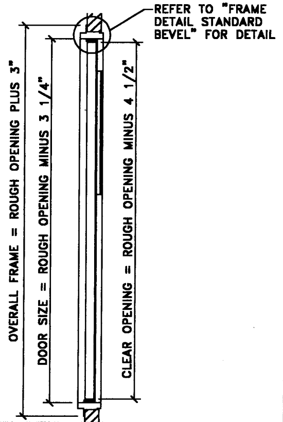
TYPICAL SECTION
